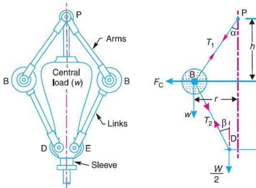
Porter governor.
