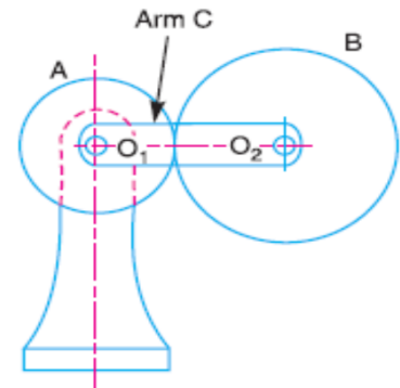
Epicyclic gear train.
